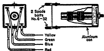
Intermediate-frequency transformer with color-coded leads.
